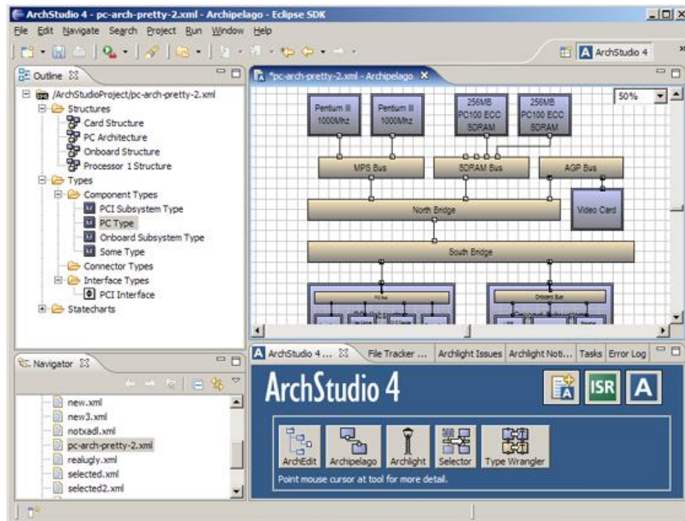
Figure 32. ArchStudio
